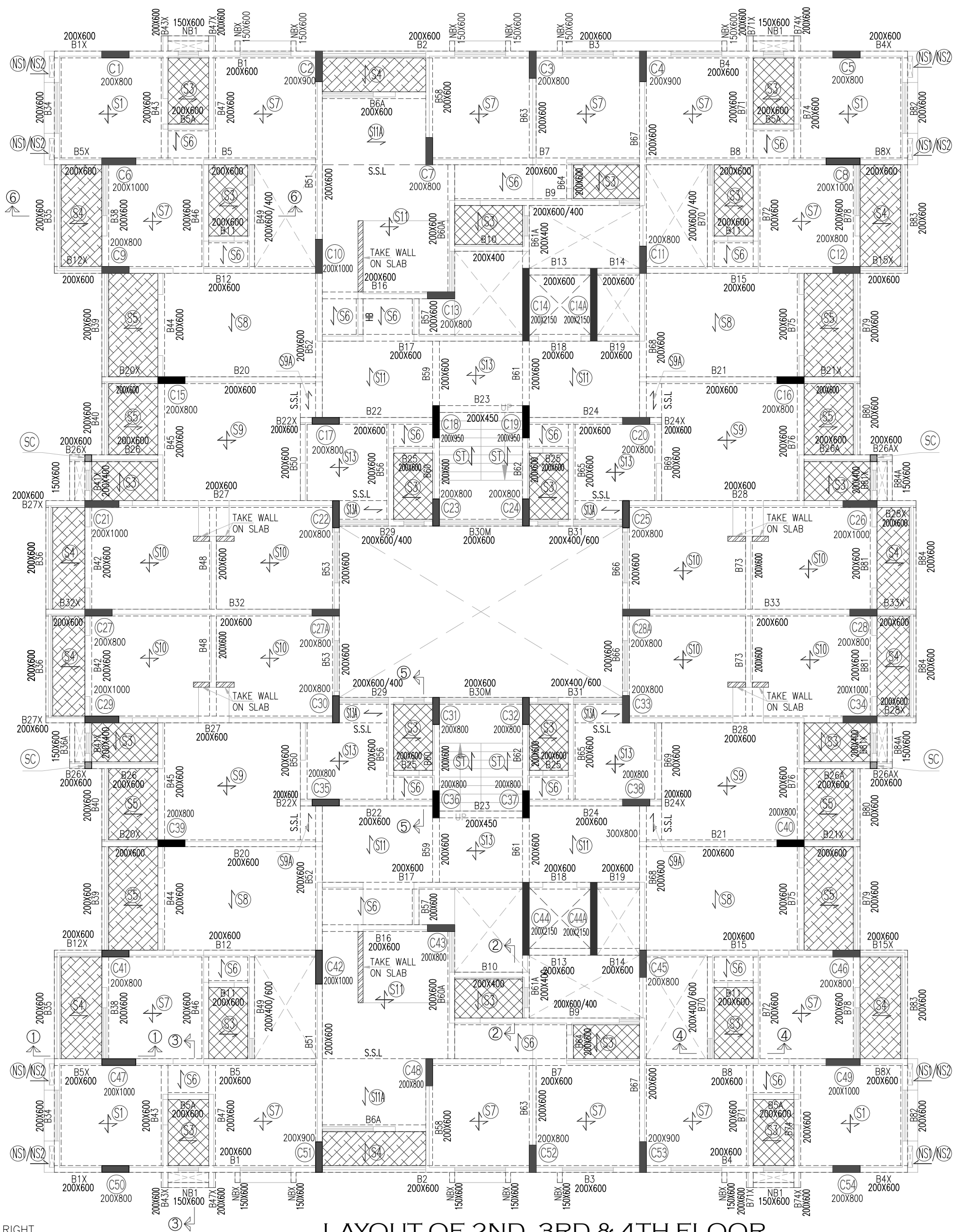
LAYOUT OF 2ND, 3RD & 4TH FLOOR BUILDING-B
